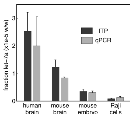
Figure 4. Experimental demonstration and validation of let-7a quantification from four total RNA samples using our two-stage ITP assay. Concentrations of let-7a in human brain (RIN = 8.2, N = 5 ), mouse brain (RIN = 8.4, N = 3 ), mouse 15 day embryo (RIN = 9.9, N = 3 ), and Raji cells (RIN = 10, N = 3 ) were measured using the ITP-based assay and an off-the-shelf Taqman RT-PCR assay. Uncertainty bars: 95 % confidence on the mean.
